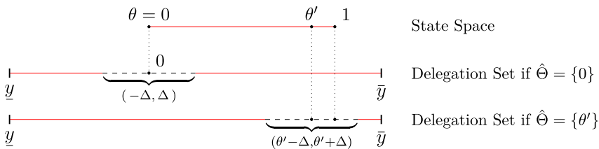
Figure 3: Illustration of Lemma 2.
