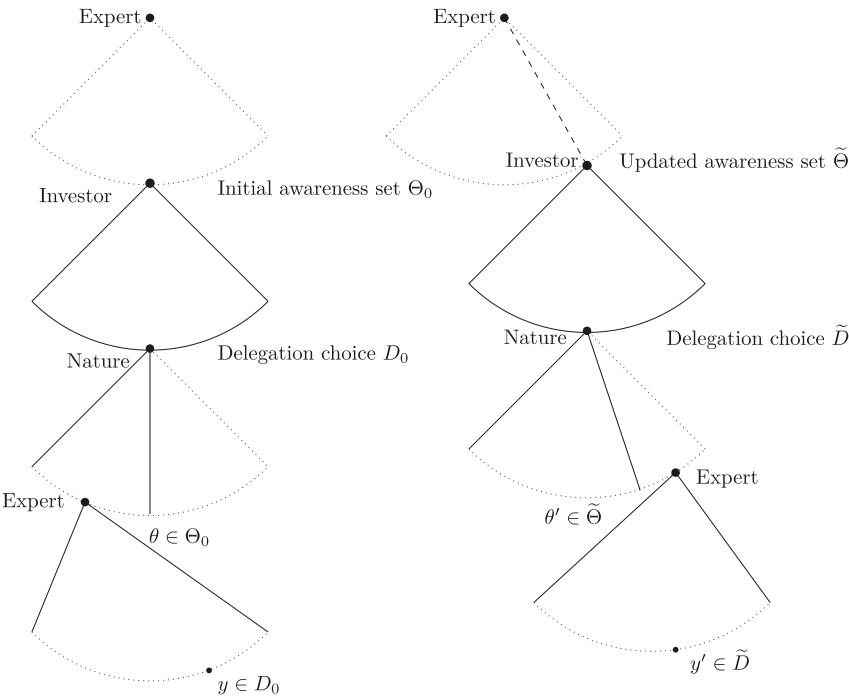
Figure 6: Subtrees T_0 and \tilde{T} .
