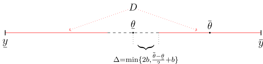
Figure 2: Delegation choice when the awareness set is [\underline{\theta}, \bar{\theta}] .
